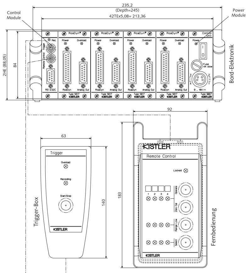
Fig. 1: Dimensions of Type 9867A... on-board electronics PremiumLine
